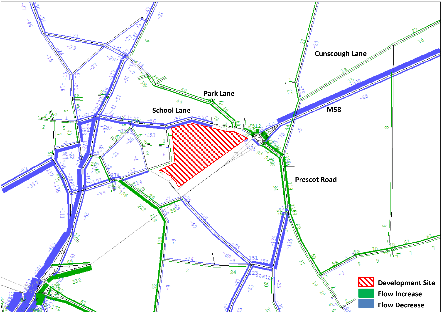
2019 Flow Comparison (PM): Do Something minus Base – Including slips – Site zoom
