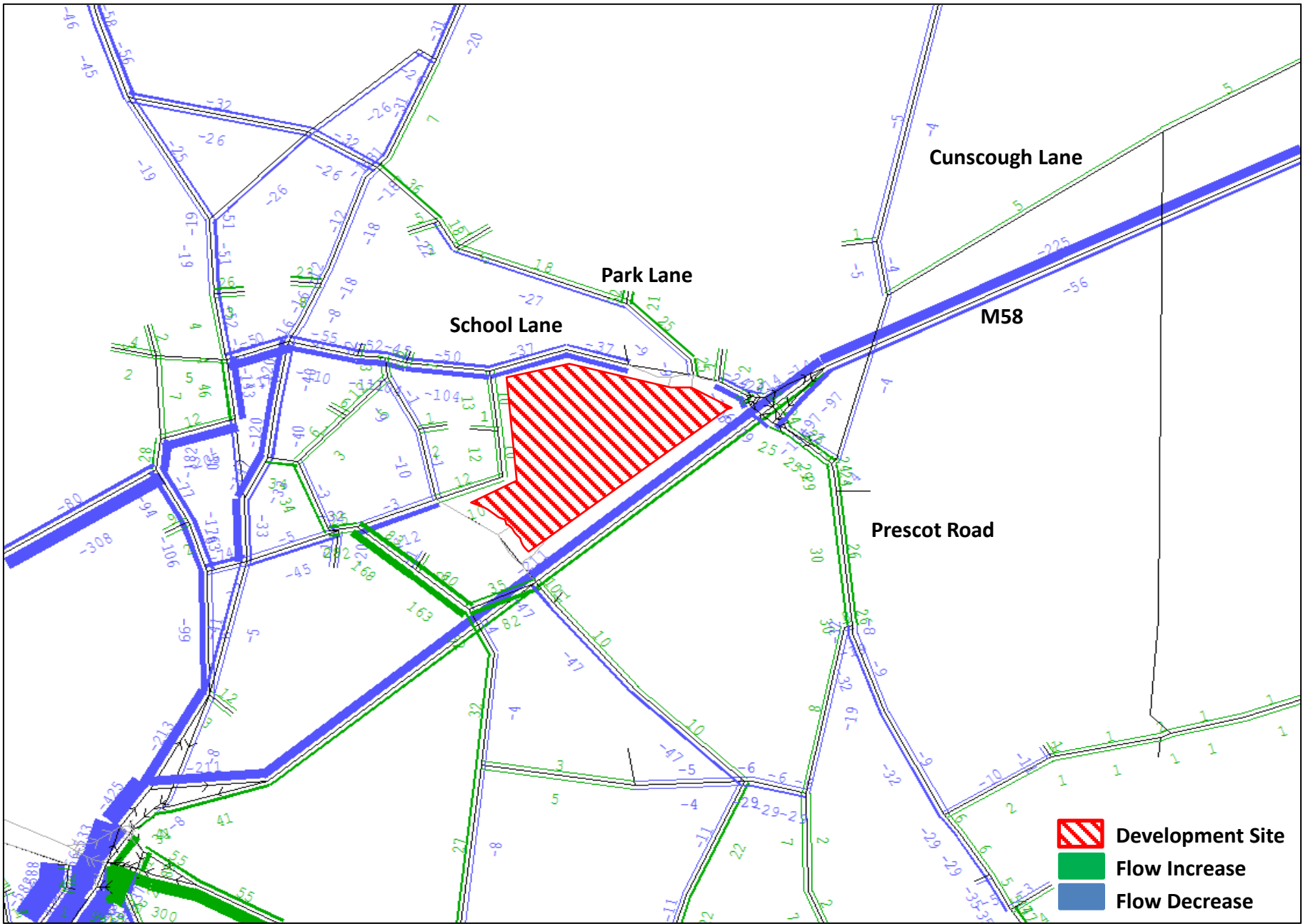
2019 Flow Comparison (PM): Do Something minus Base – Without slips - Site zoom
