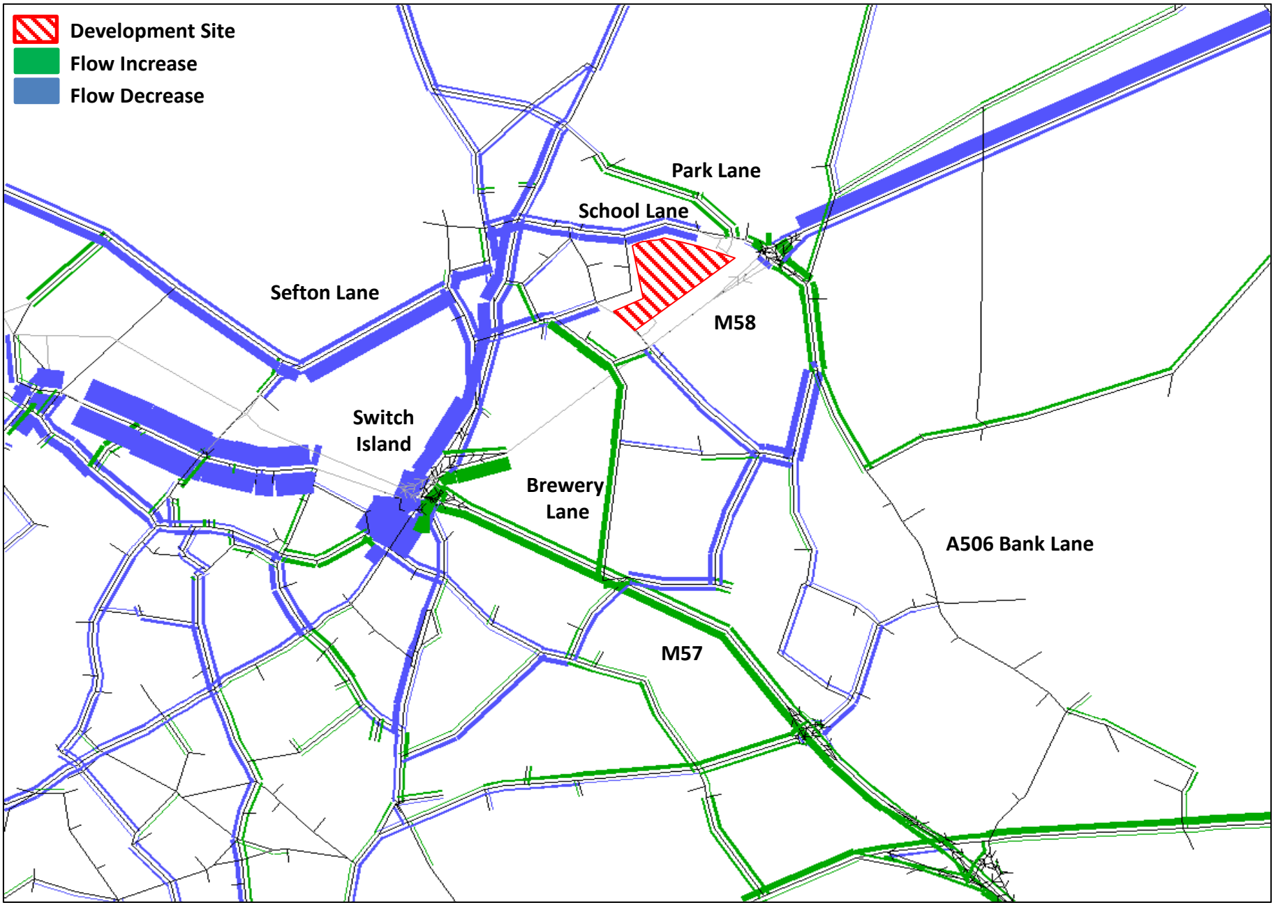
2019 Flow Comparison (PM): Do Something minus Base – Including slips
