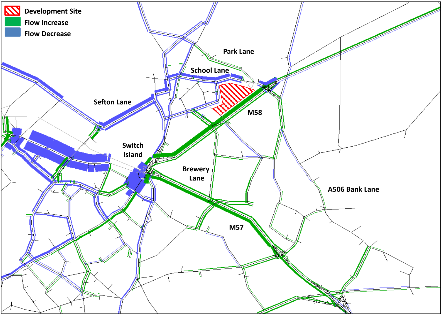
2019 Flow Comparison (AM): Do Something minus Base – Without slips
